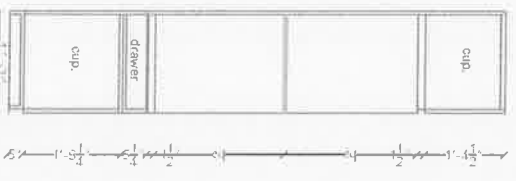
DRAWER SECTION
