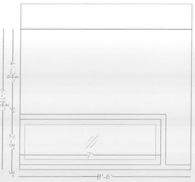
FRONT PARTITION
