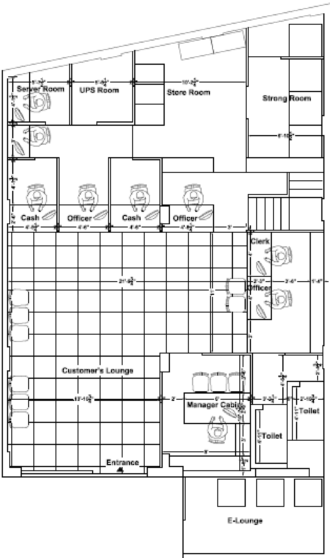
INTERIOR LAYOUT GROUND FLOOR OF VASCO DA GAMA BRANCH FOR BANK OF MAHARASHTRA
