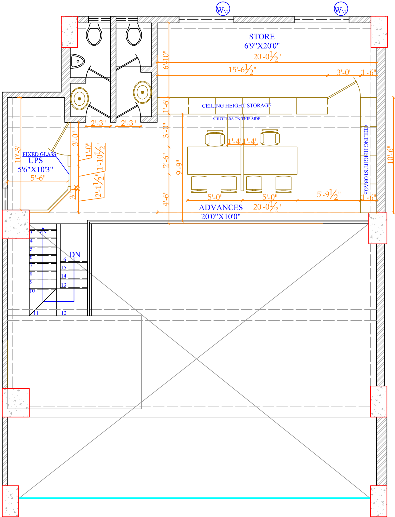
MEZZANINE PLAN
