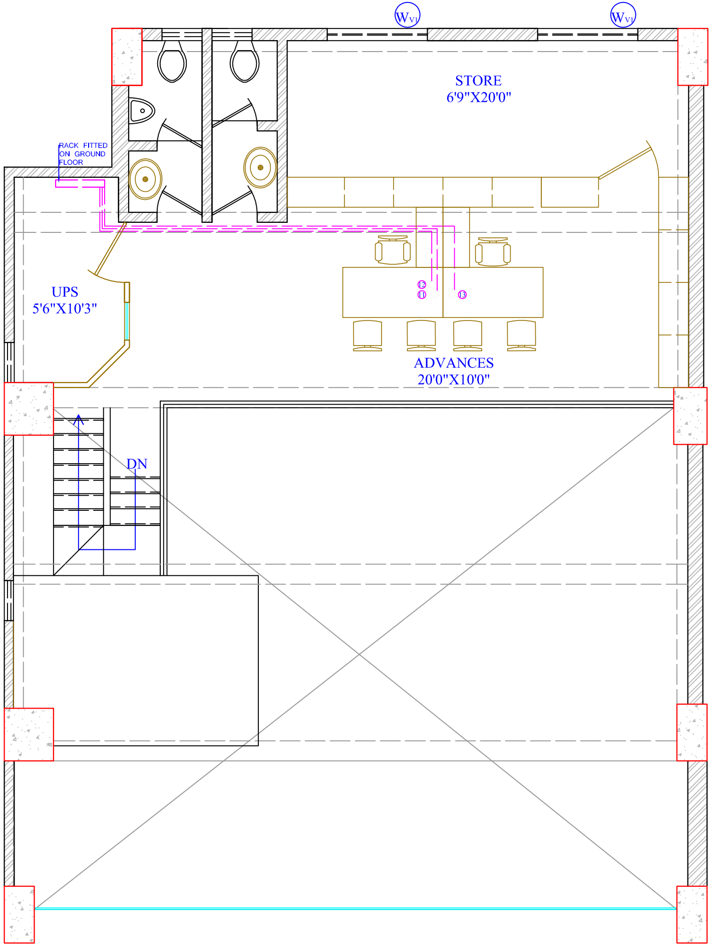
MEZZANINE PLAN
