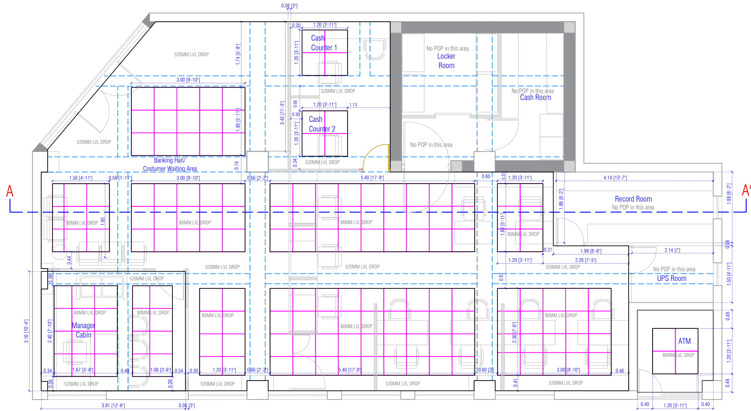
CEILING LAYOUT- for MAIN BRANCH OFFICE
