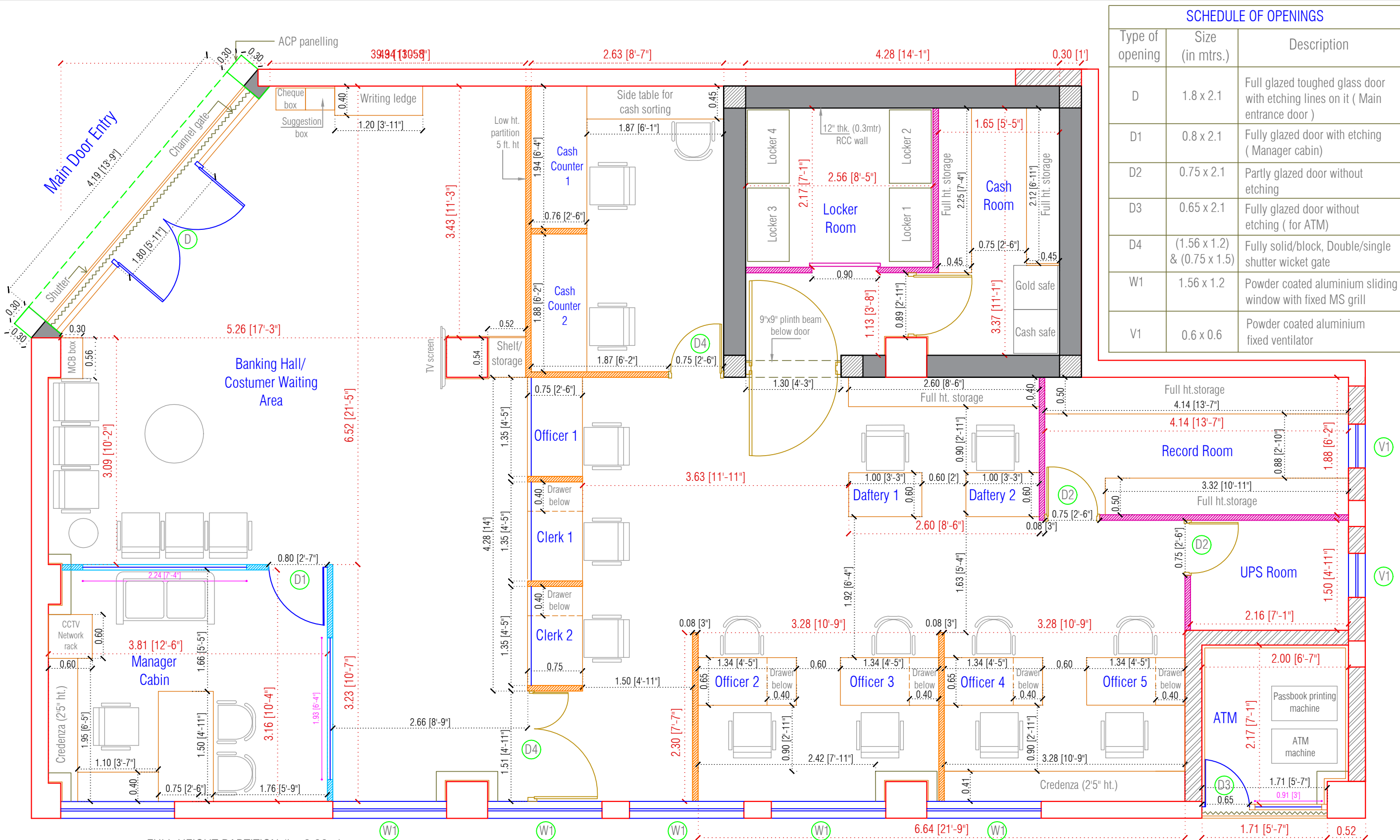
PLAN- for MAIN BRANCH OFFICE CARPET AREA = 146.40 SQ.M. (1575.84 SQ.FT.)
