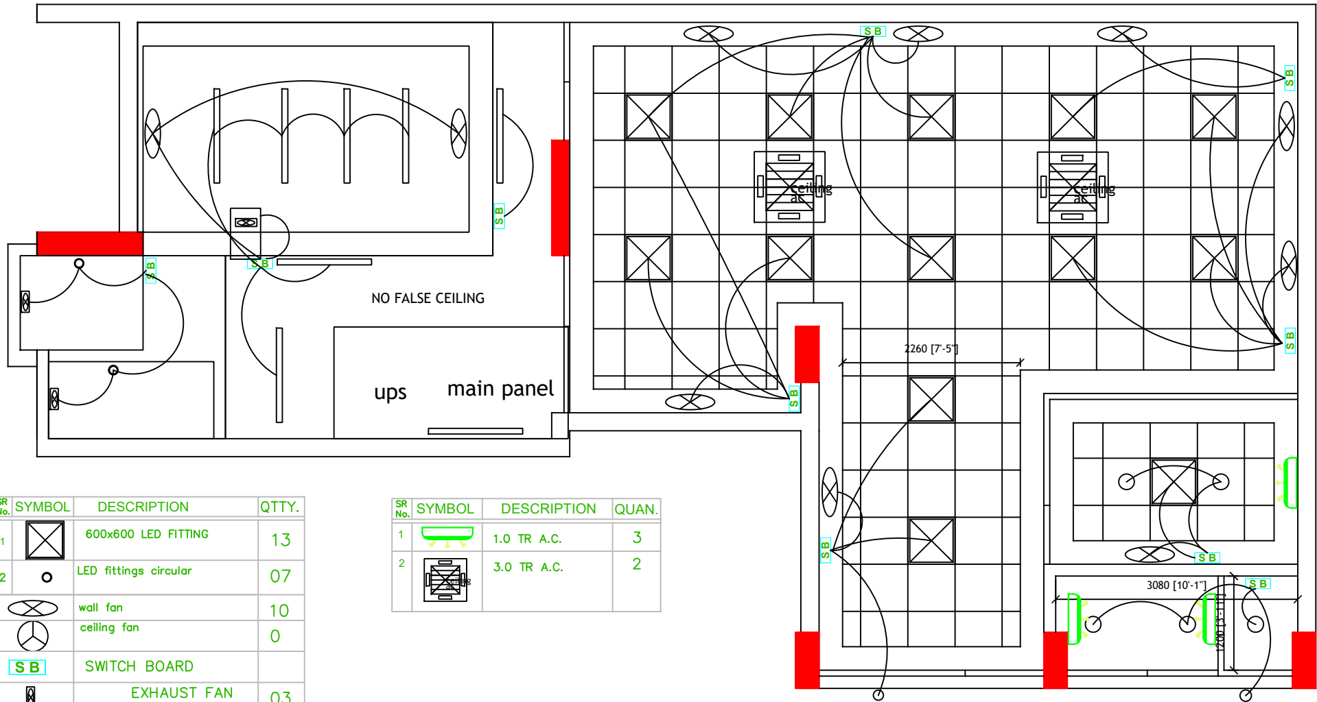
CEILING LAYOUT
